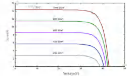
I-V/P-V Curve at Different Irradiation (480W)
