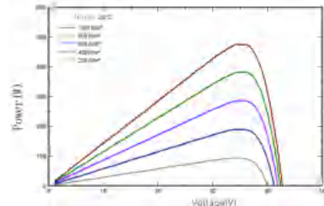
I-V/P-V Curve at Different Irradiation (480W)
