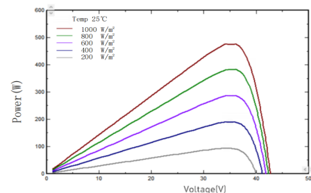
I-V/P-V Curve at Different Irradiation (480W)
